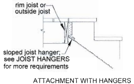
Figure 31: Stair Stringer Attachment Detail
