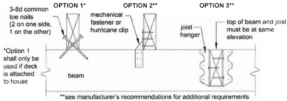
Figure 6: Joist-to-Beam Detail
