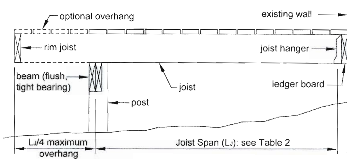
Figure 1A: Joist Span – Deck Attached at House and Bearing Over Beam
