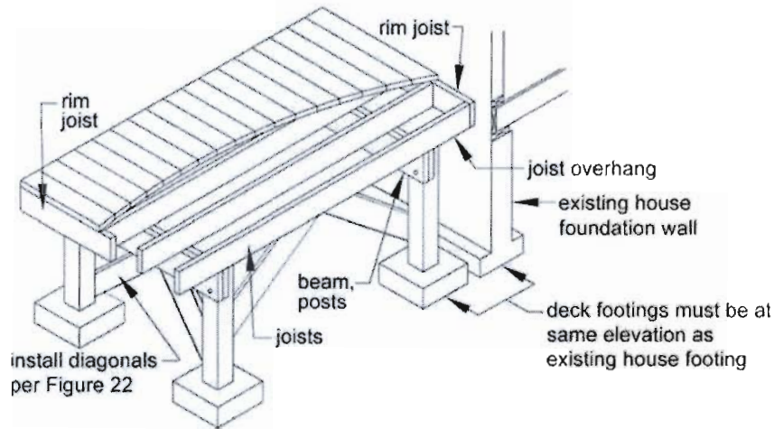
Figure 21: Free-Standing Deck
